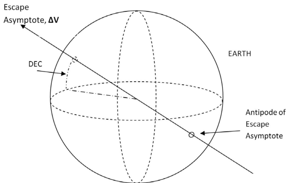
Figure 4 The Escape Aymptote Direction and its Declination
